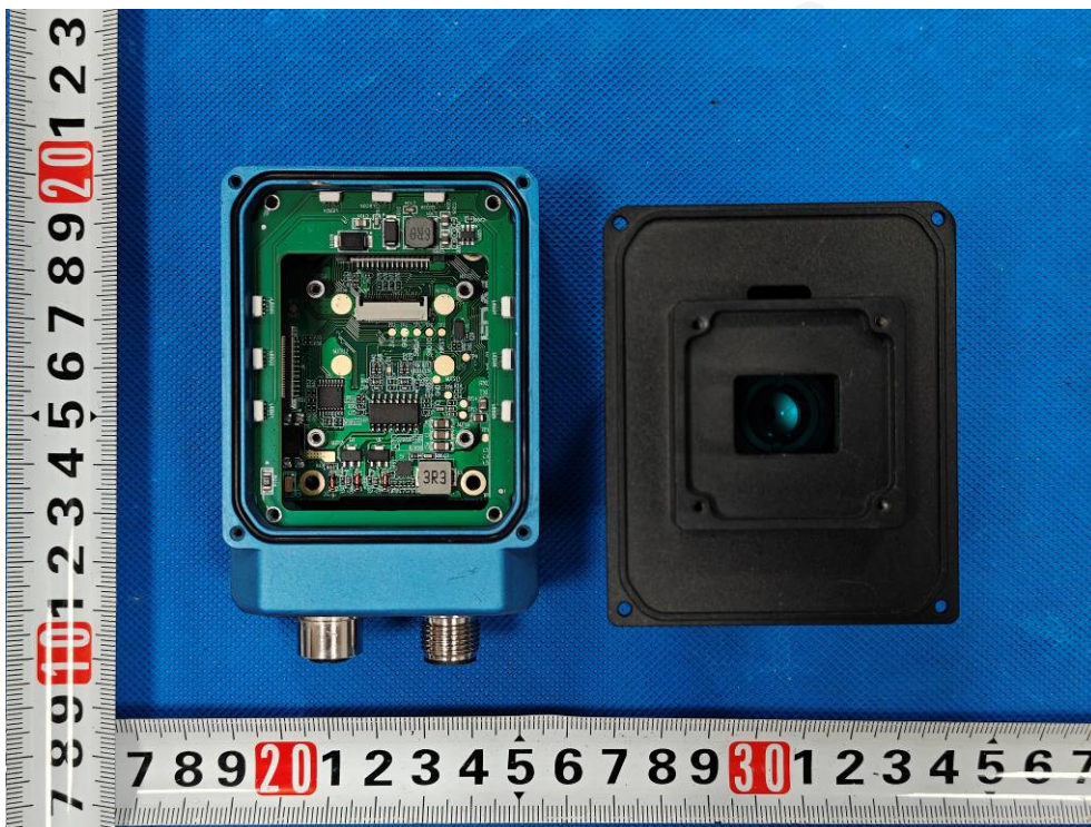
Photo 8: Internal view - ED-AIC3100
