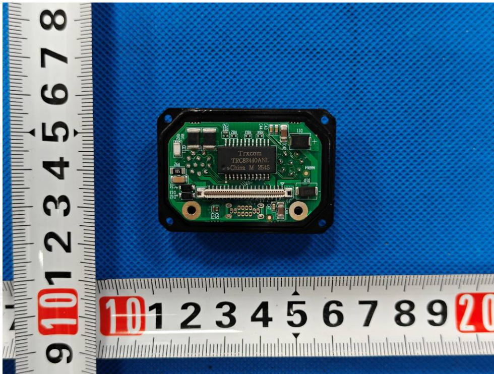
Photo 17: PCB view - ED-AIC3100
