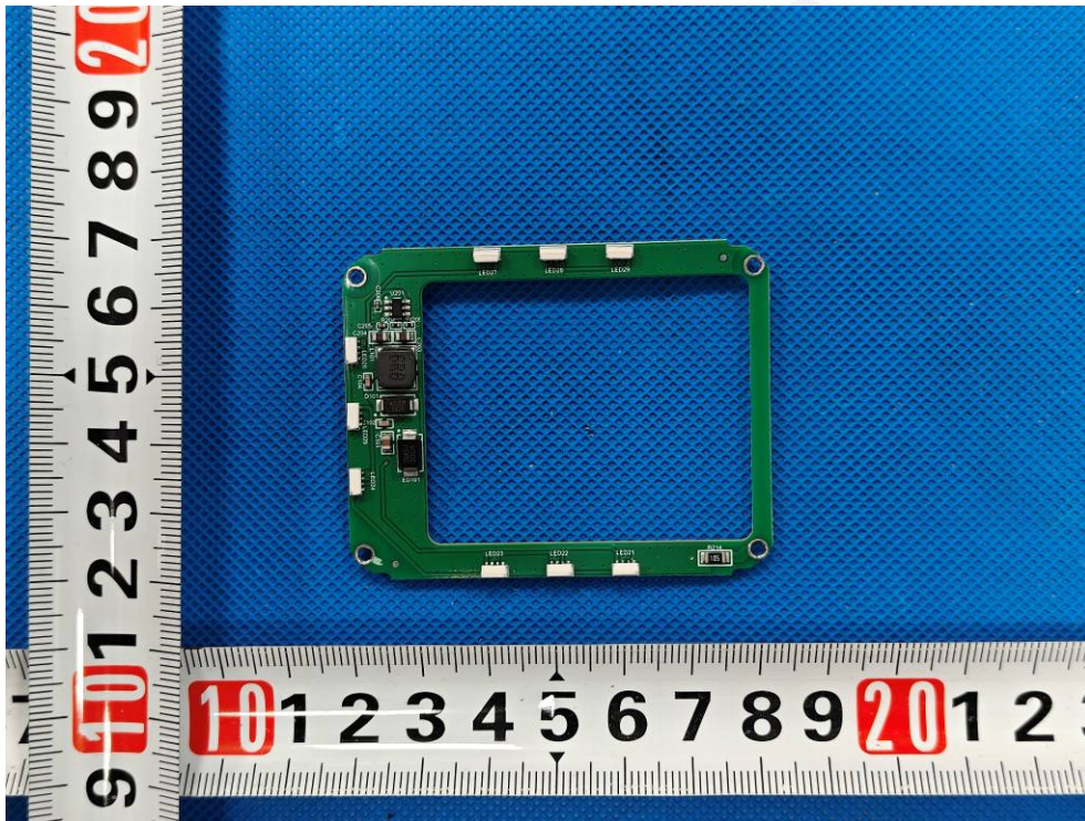
Photo 14: PCB view - ED-AIC3100
