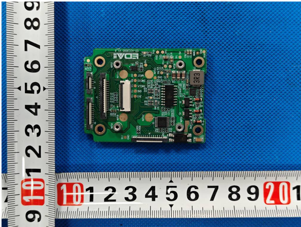
Photo 10: PCB view - ED-AIC3100
