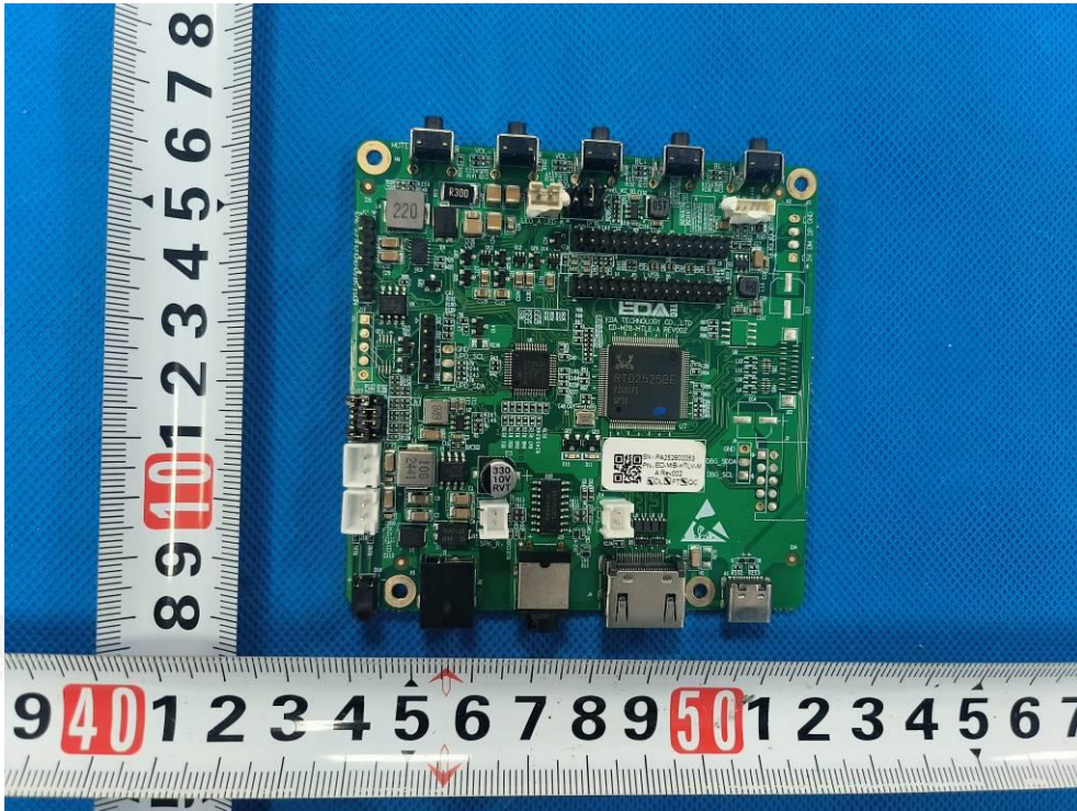
Photo 11: PCB view for model ED-MONITOR-215CA
