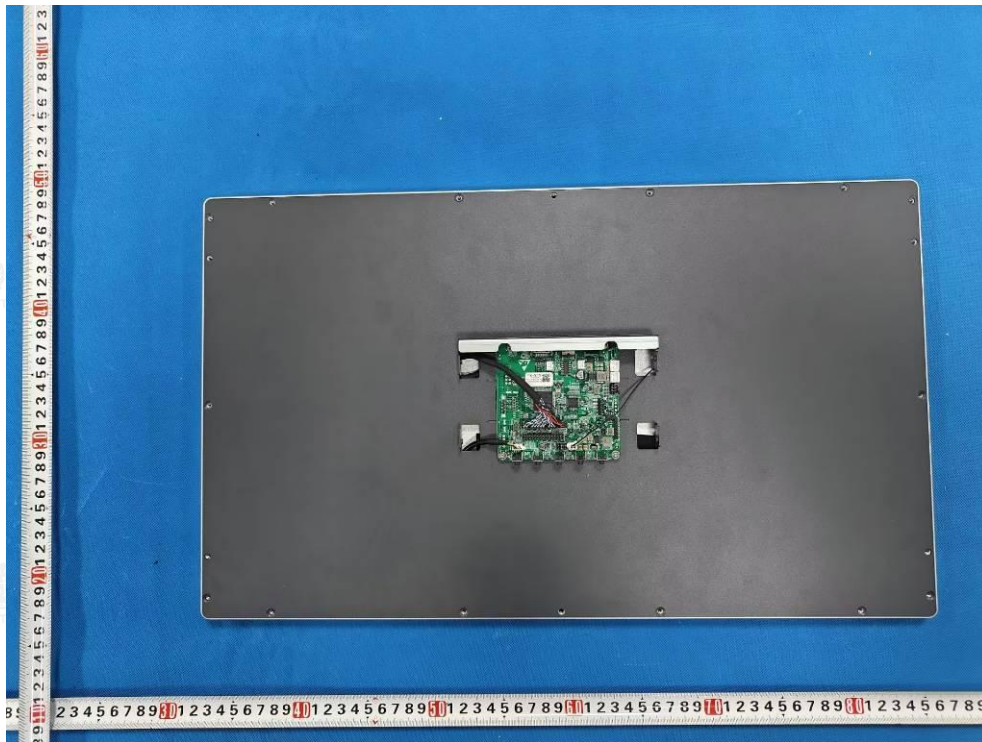
Photo 9: Internal view for model ED-MONITOR-215CA
